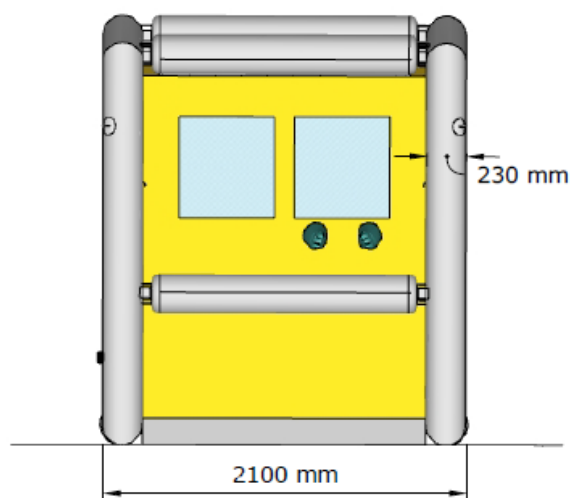
LEFT VIEW
